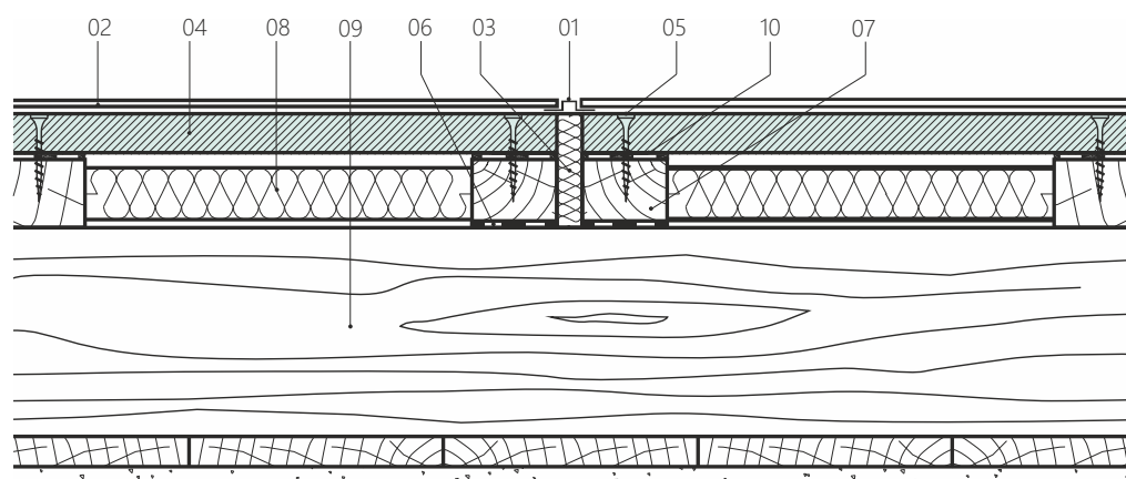
Floor boards on beams – solution of dilatation
