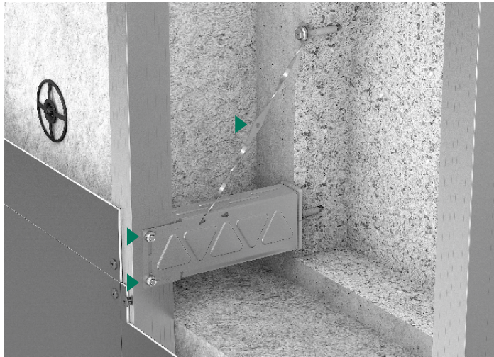
Fixed point: Fixing in a circular hole, completed by a hinge for reliable transfer of own weight.
