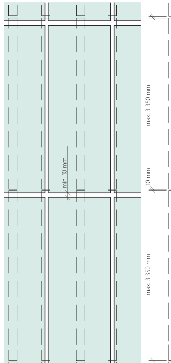
Dilatation – grid of aluminium or zinc-coated profiles
