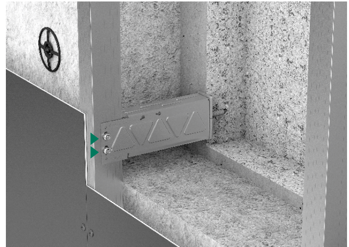
Sliding point: Fixing in the oval hole.
