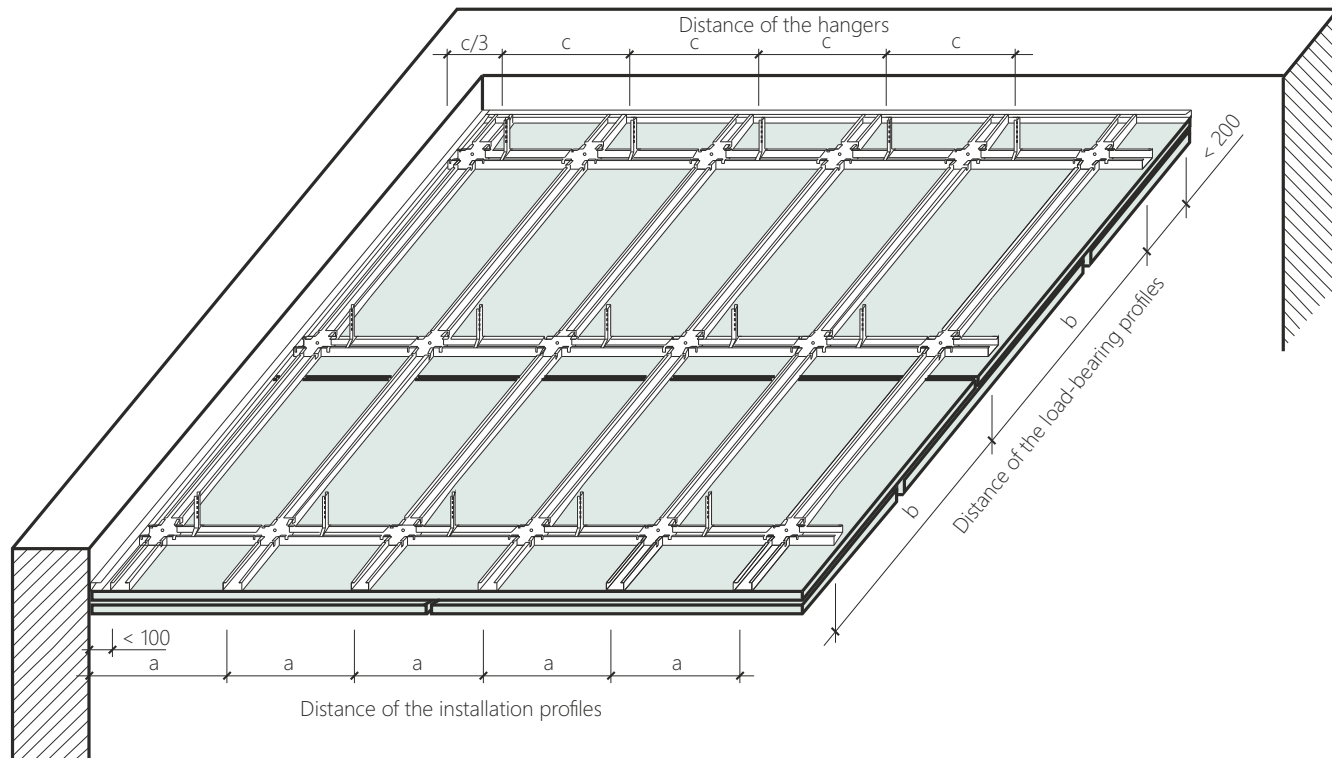
Fig. 2) Schematic drawing of the load-bearing construction of the ceiling for cladding with CETRIS® cement bonded particleboard (thickness 2 \times 12 mm)
