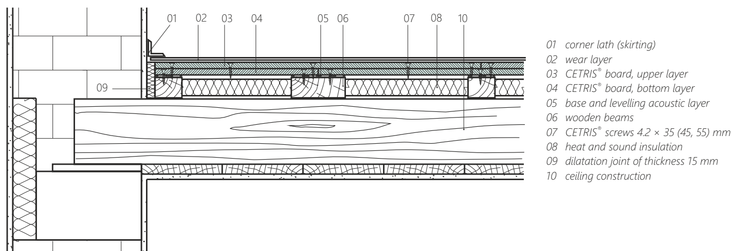
Two-layer CETRIS® board floors on beams
