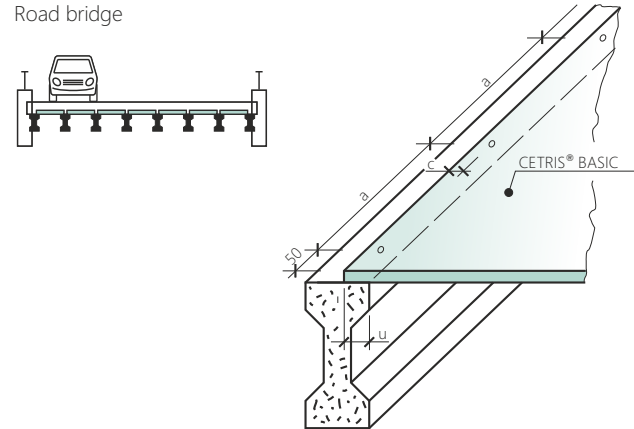
Road bridge
